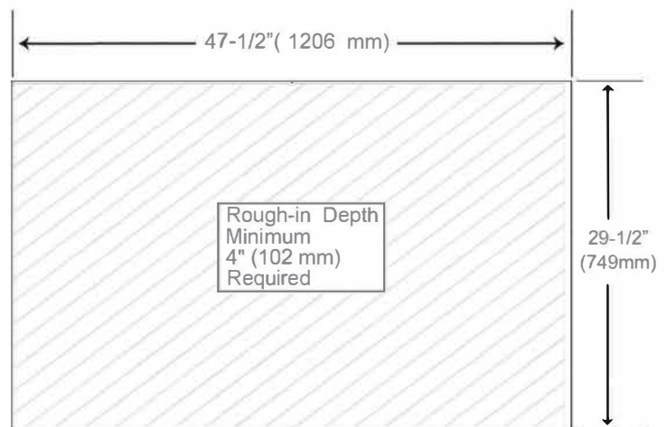
Rough-in Dimensions
