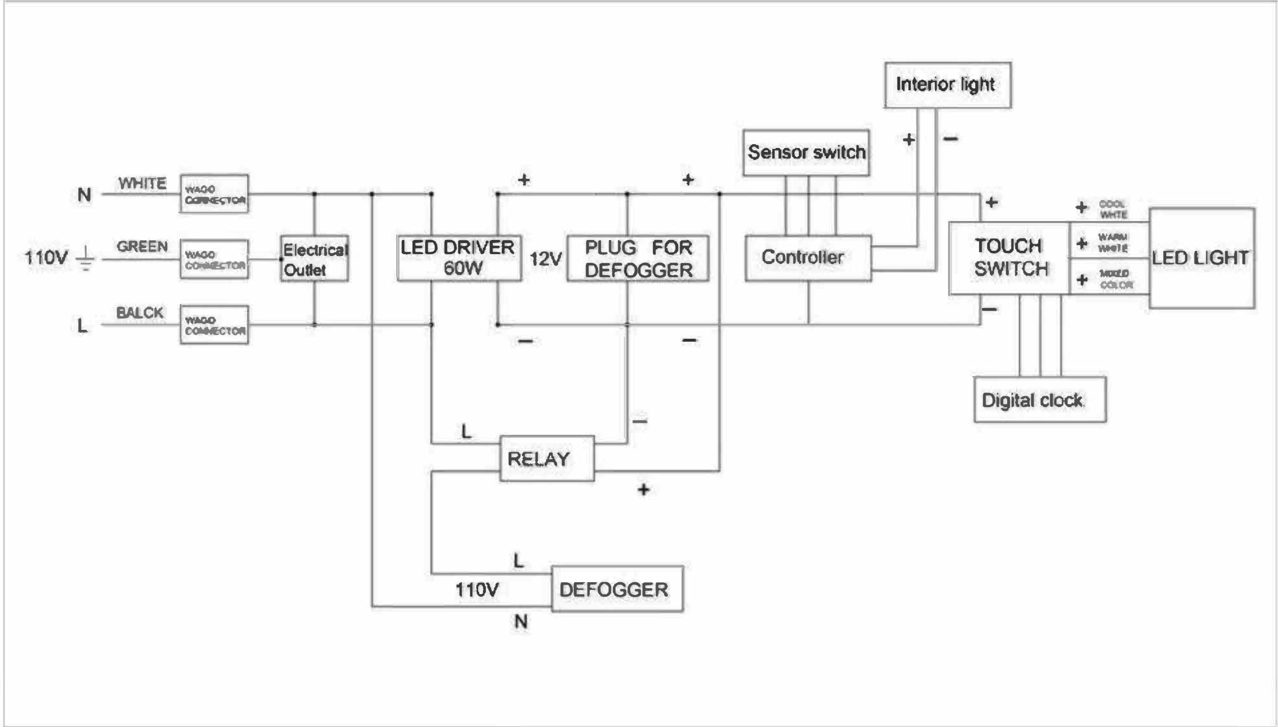
Circuit Diagram
