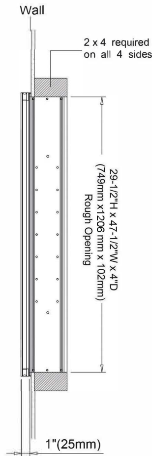
Recessed Mount
