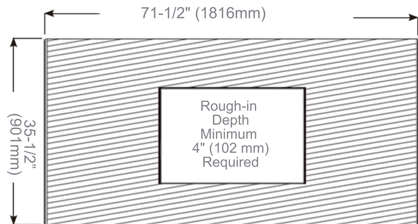
Rough-in Dimensions
