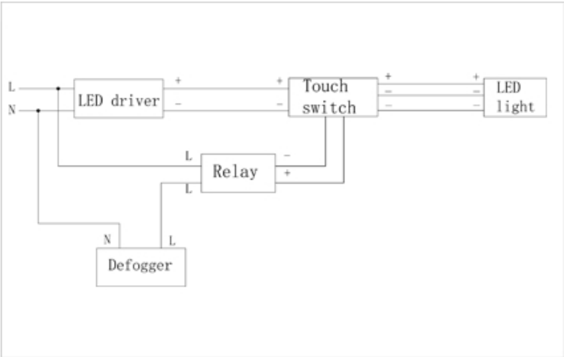
Circuit diagram
